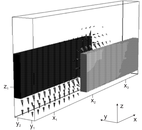
Figure 1: Elementary comb cell with two half fingers
